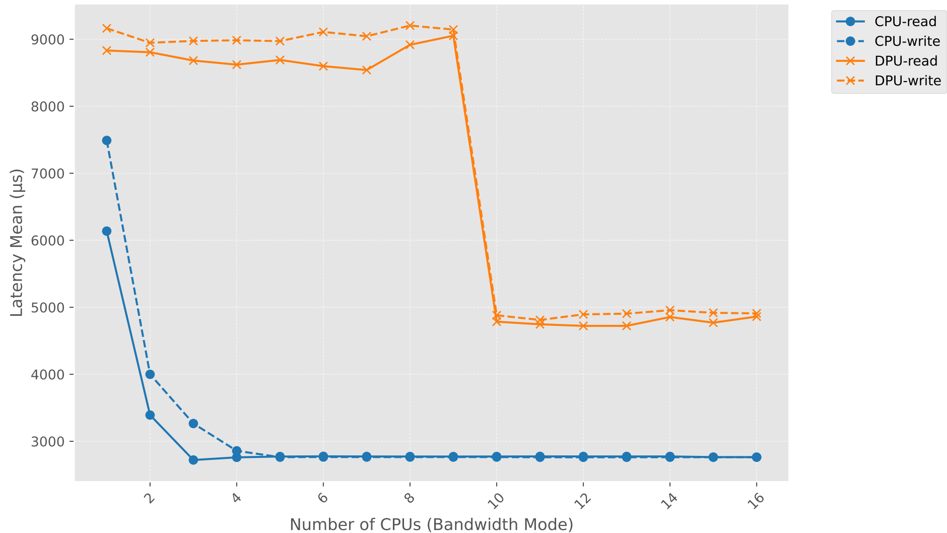
Latency Mean vs Number of CPUs (Bandwidth Mode)
